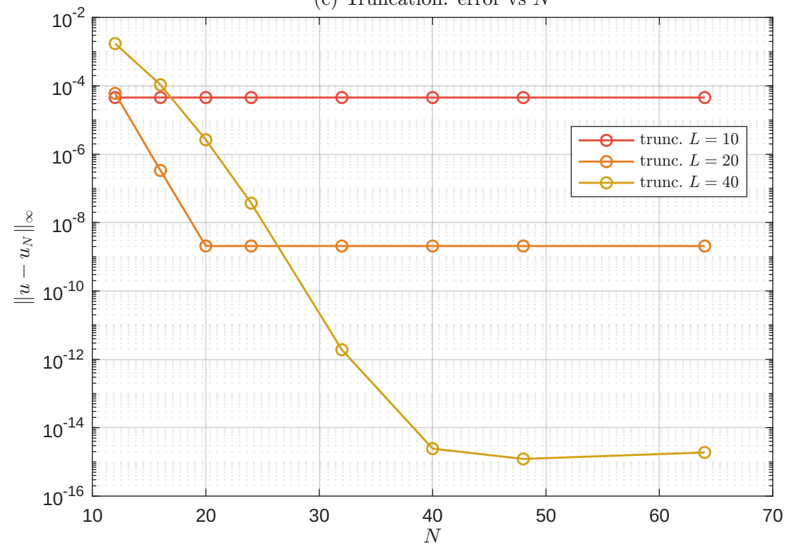
(c) Truncation: error vs N
