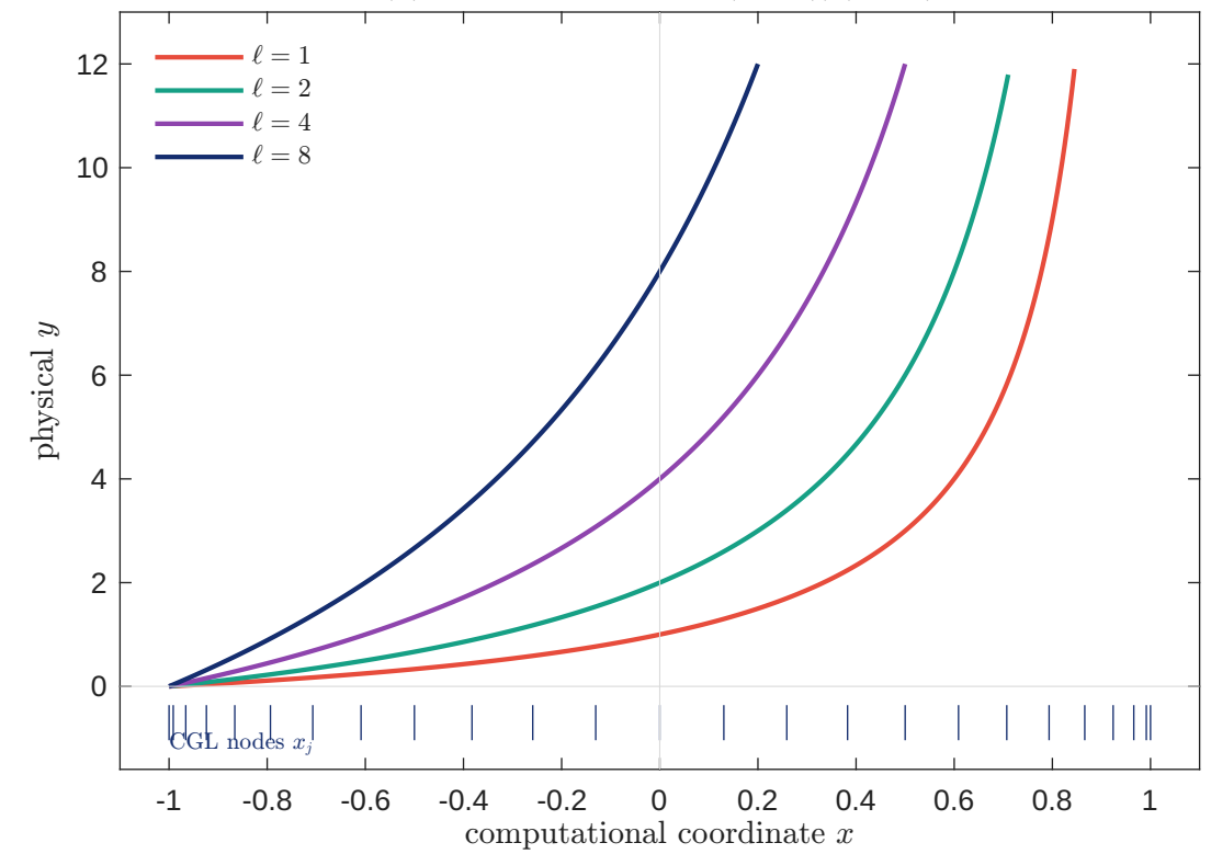
(b) Algebraic map y = \ell(1+x)/(1-x)
