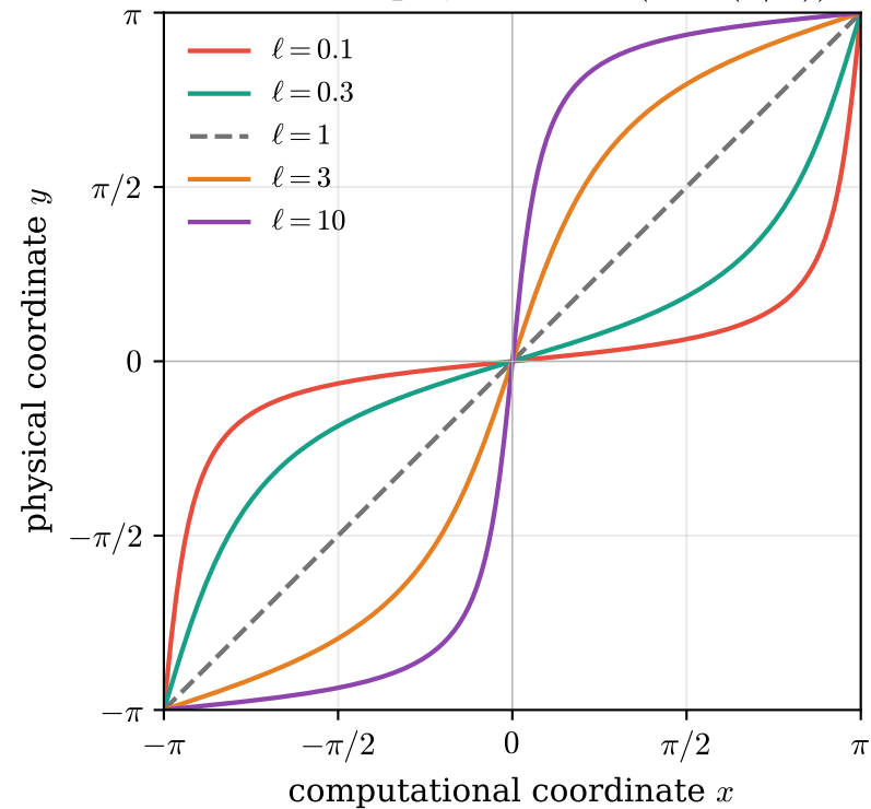
(a) the map y = 2 \arctan(\ell \tan(x/2))
