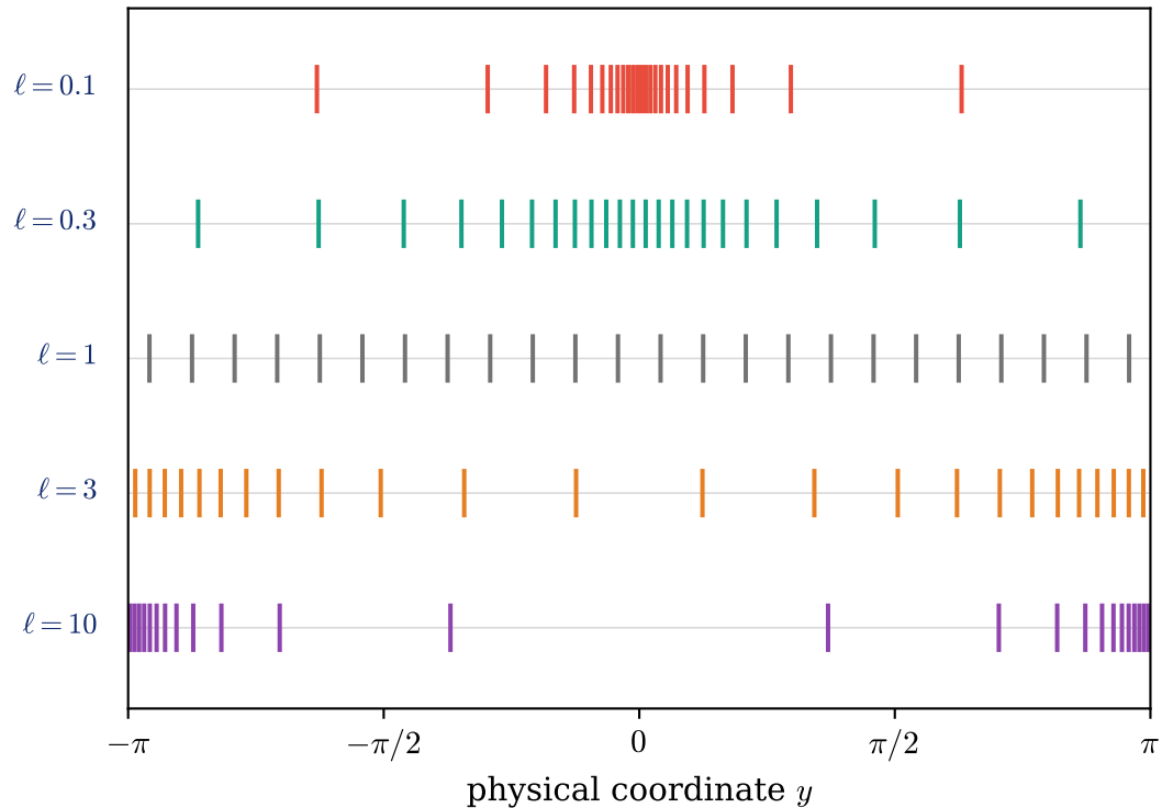
(b) image of a uniform N = 24 x -grid
