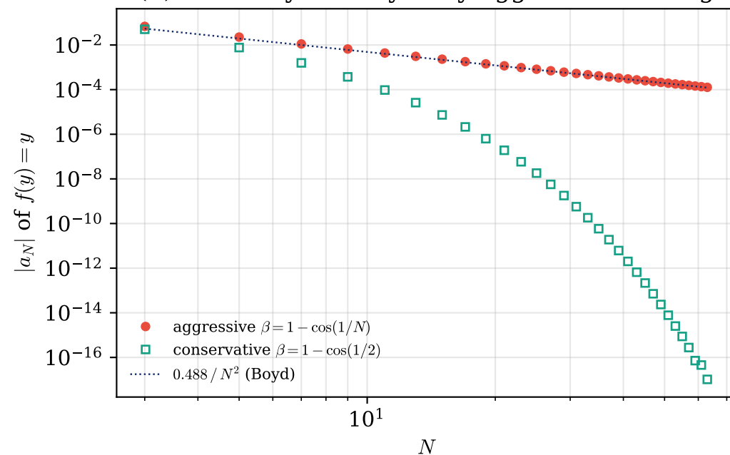
(d) Accuracy destroyed by aggressive scaling
