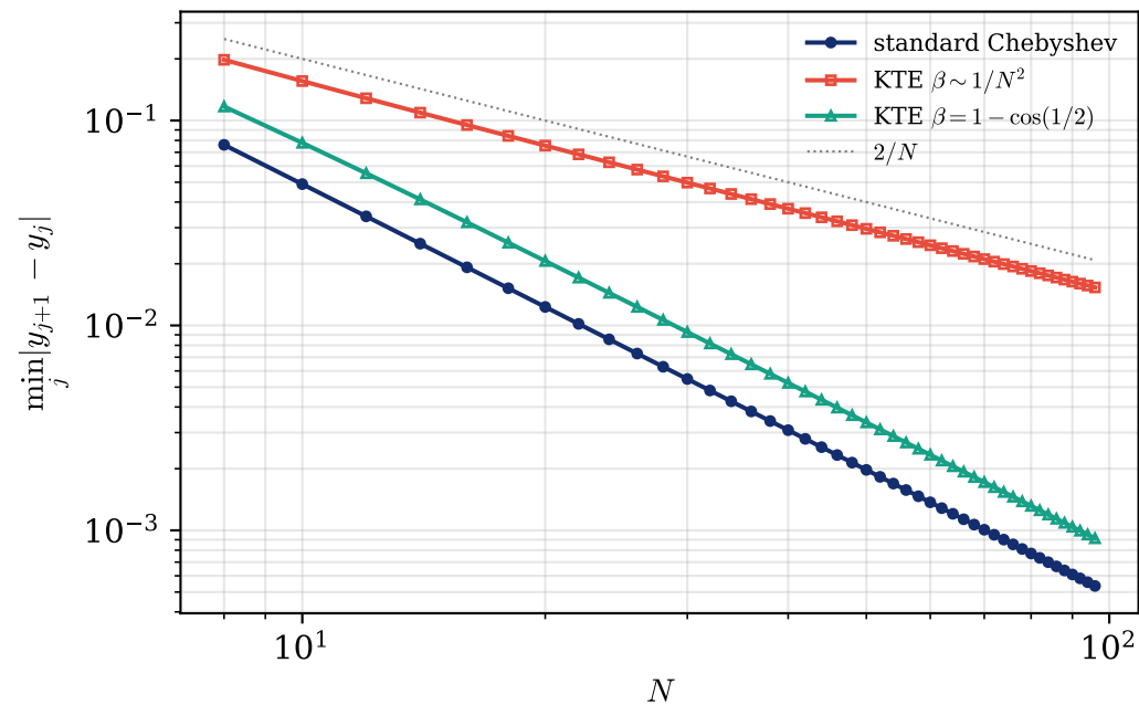
(b) Minimum spacing vs N
