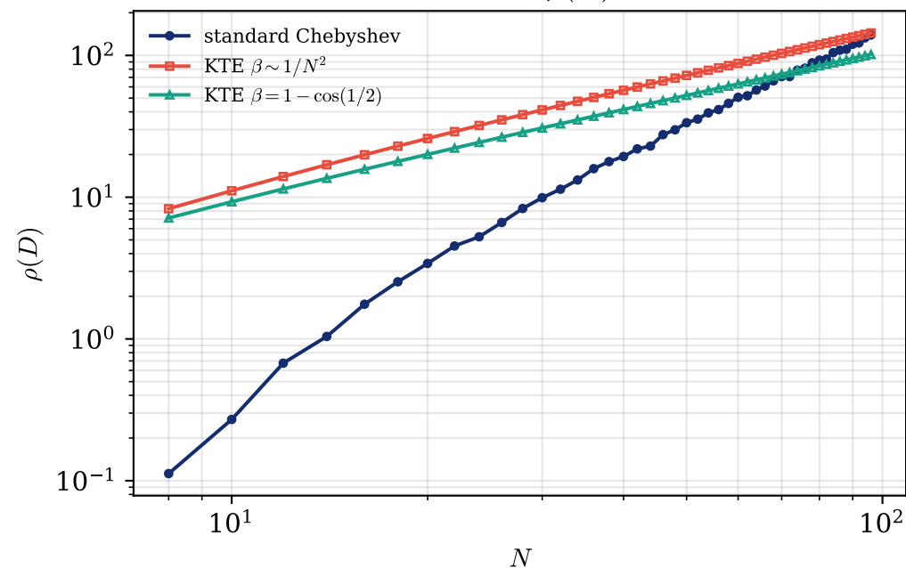
(c) Stiffness \rho(D) vs N
