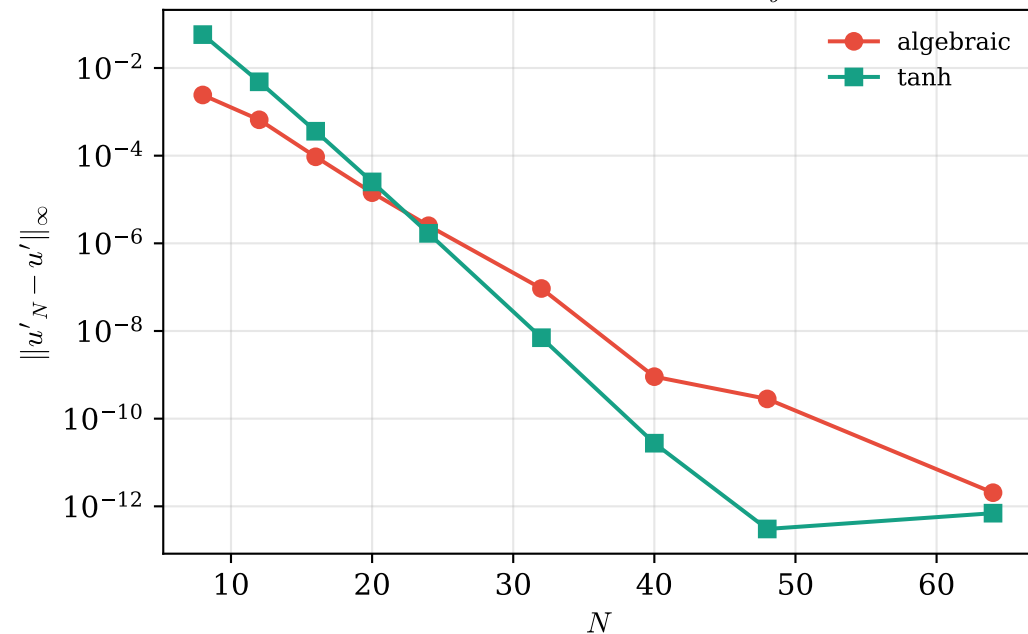
(c) First derivative: D_y u
