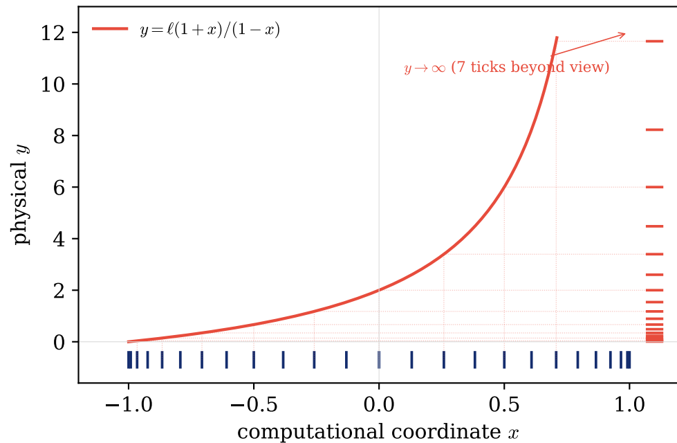
(b) algebraic map ( \ell = 2 ): clusters near y = 0
