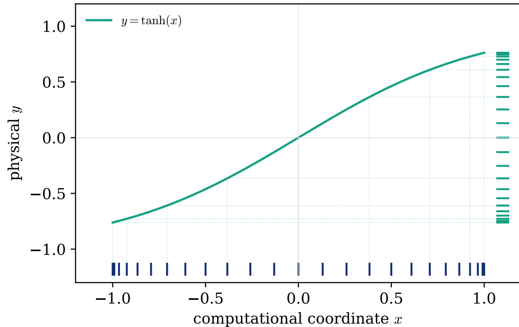
(a) tanh map: x_j (bottom) \rightarrow y_j (right)
