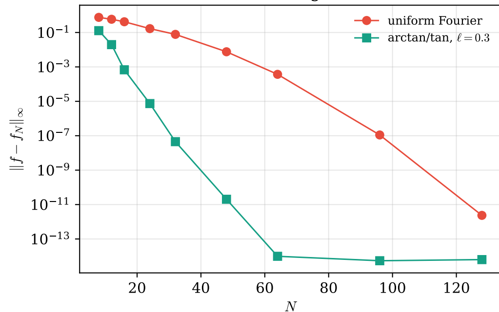
(c) Convergence
