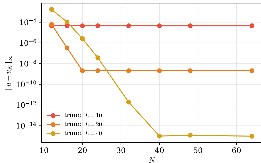
(c) Truncation: error vs N
