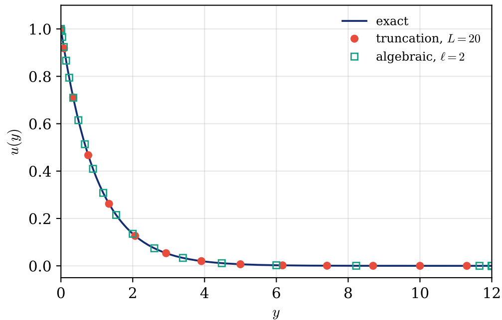
(a) Solution at N=24
