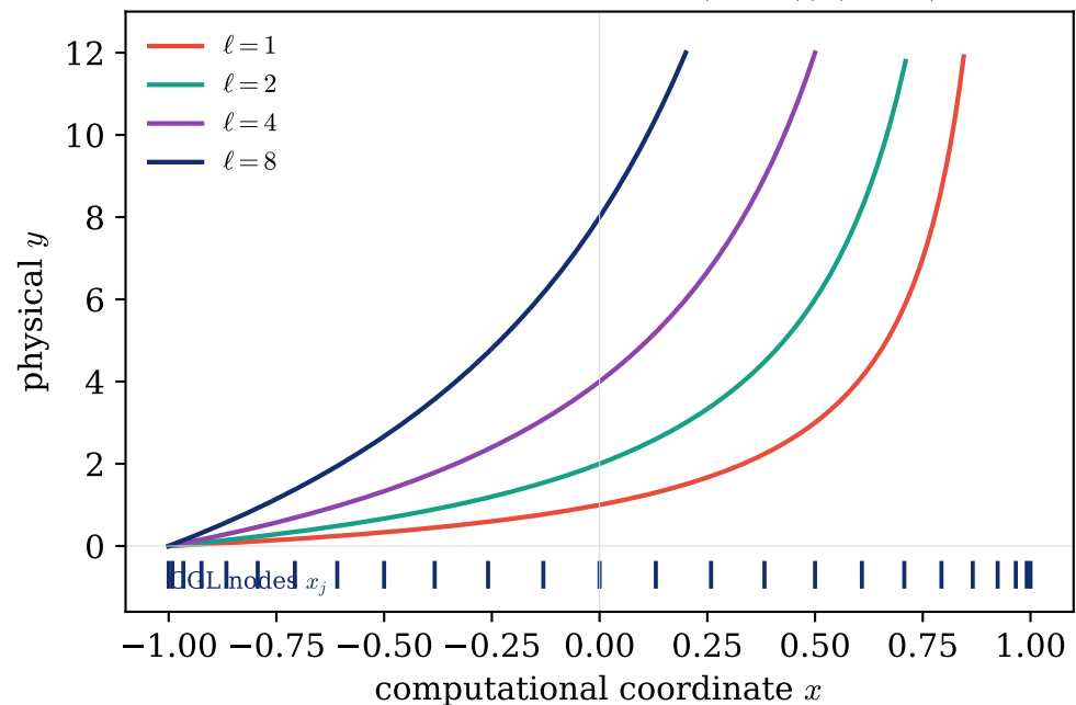
(b) Algebraic map y = \ell(1+x)/(1-x)
