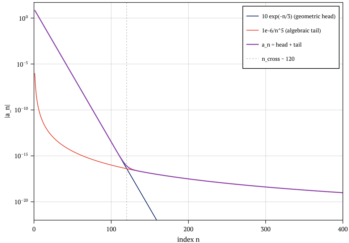
Panel A. Boyd's cartoon: slope change at n_{\text{cross}}
