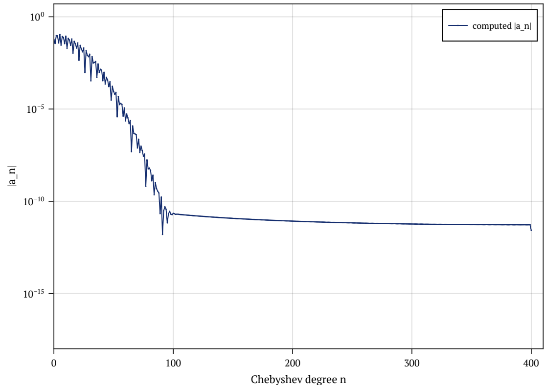
Panel B. f(x) = e^{-((x-0.3)/0.1)^2} + 1e-7 (x+1)^{1/3}
