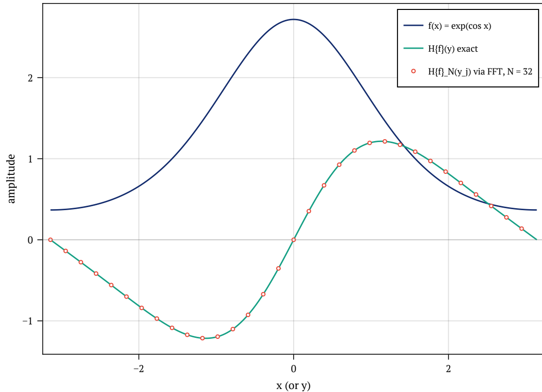
f(x) = \exp(\cos x) and its Hilbert transform on the circle
