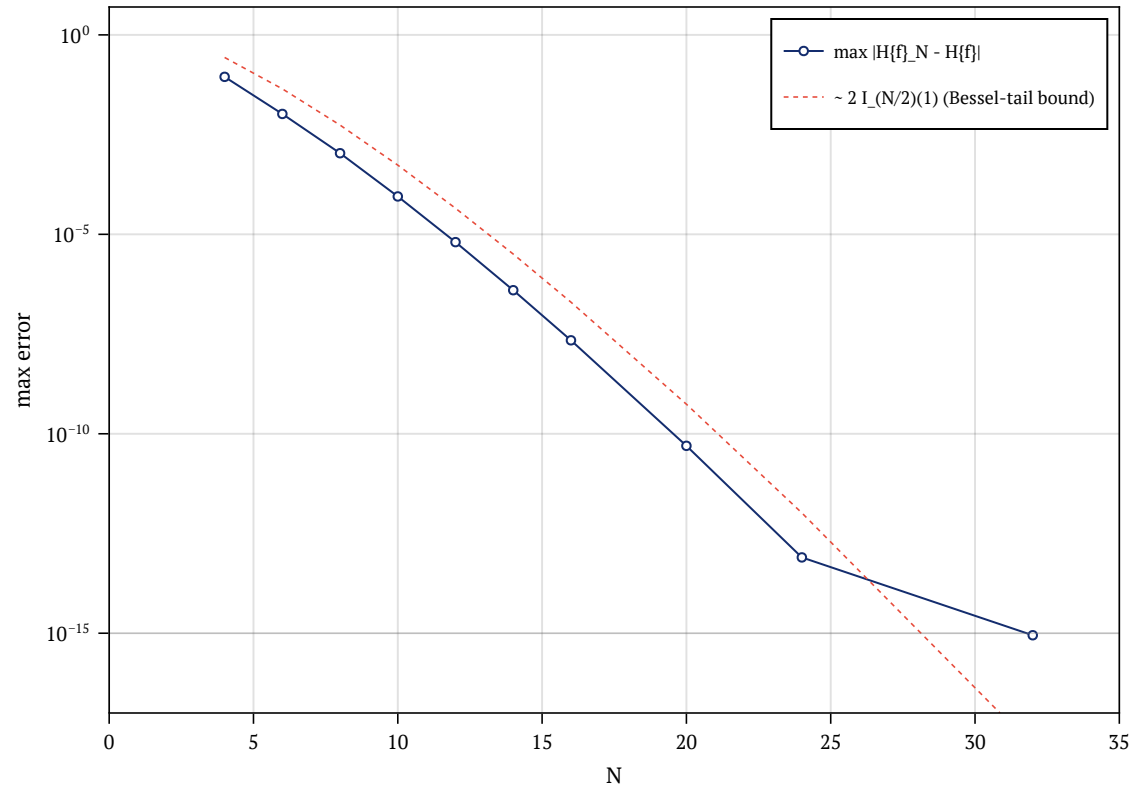
super-geometric convergence on a periodic test
