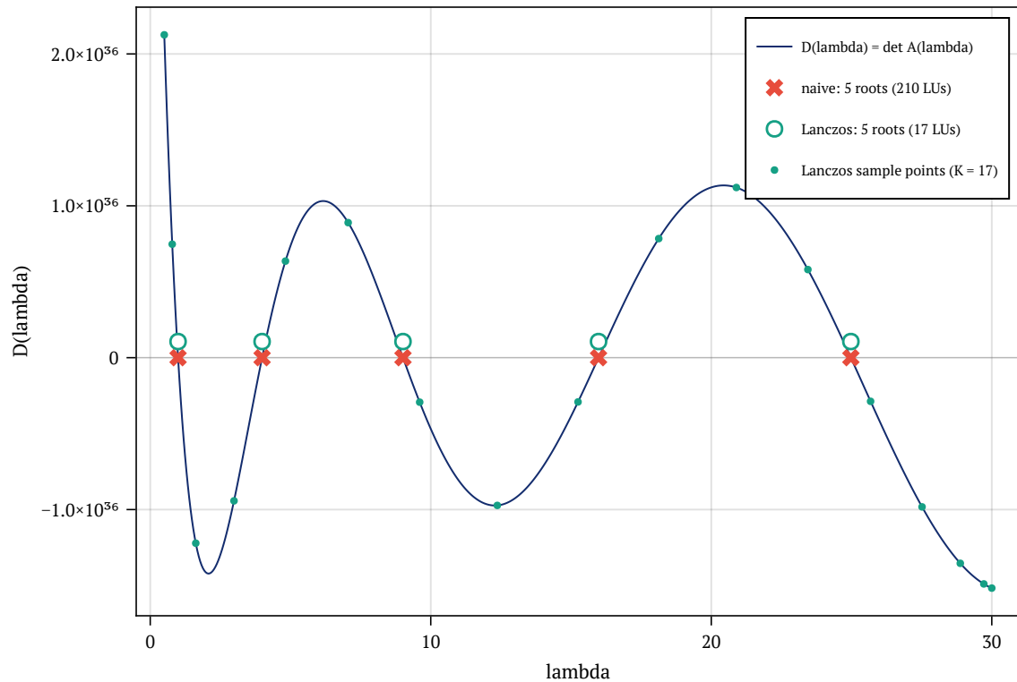
the determinant and the two strategies' detected roots
