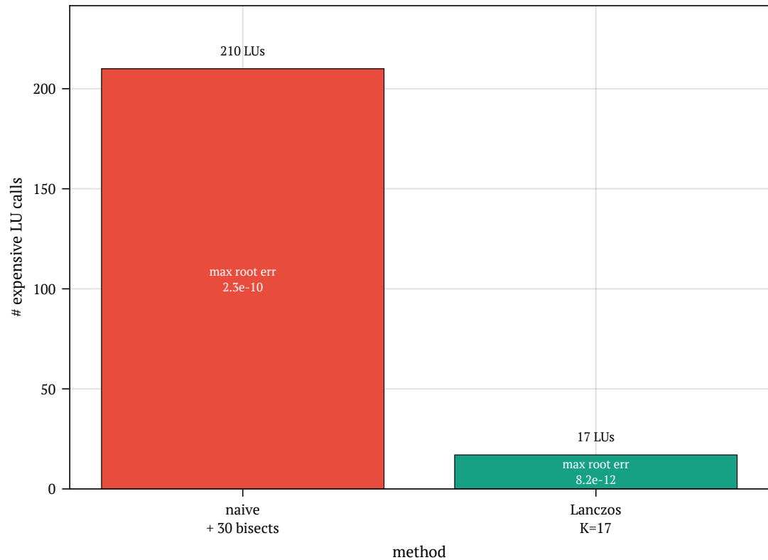
cost: 17 vs 210 LU factorisations
