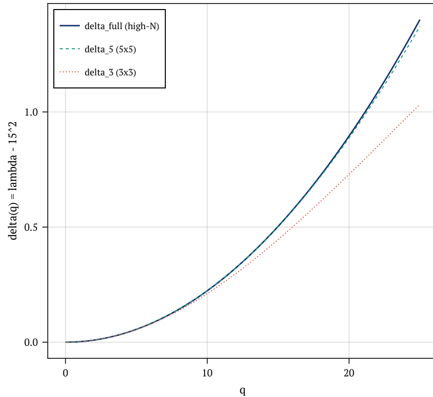
Panel B. ce_15: 5x5 matches full to plot accuracy
