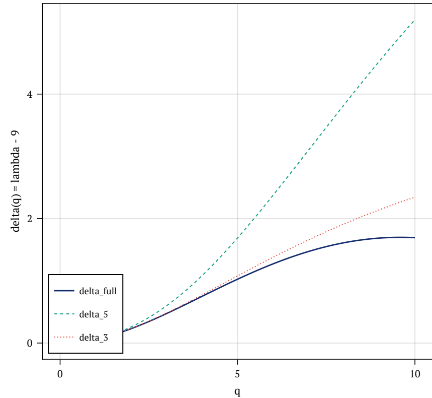
Panel C. ce_3: q/n^2 large, sideband breaks
