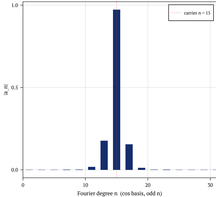
Panel A. |a_n| for ce_15 at q = 10.0
