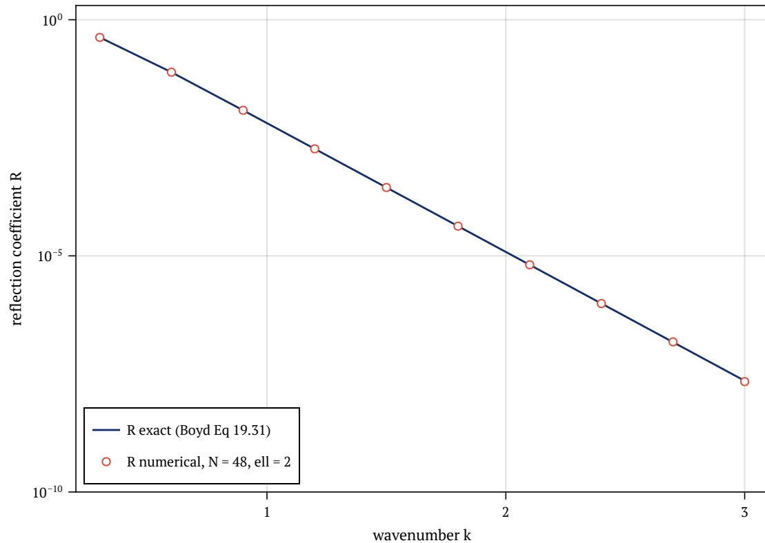
sech 2 scattering: spectral R matches the closed form
