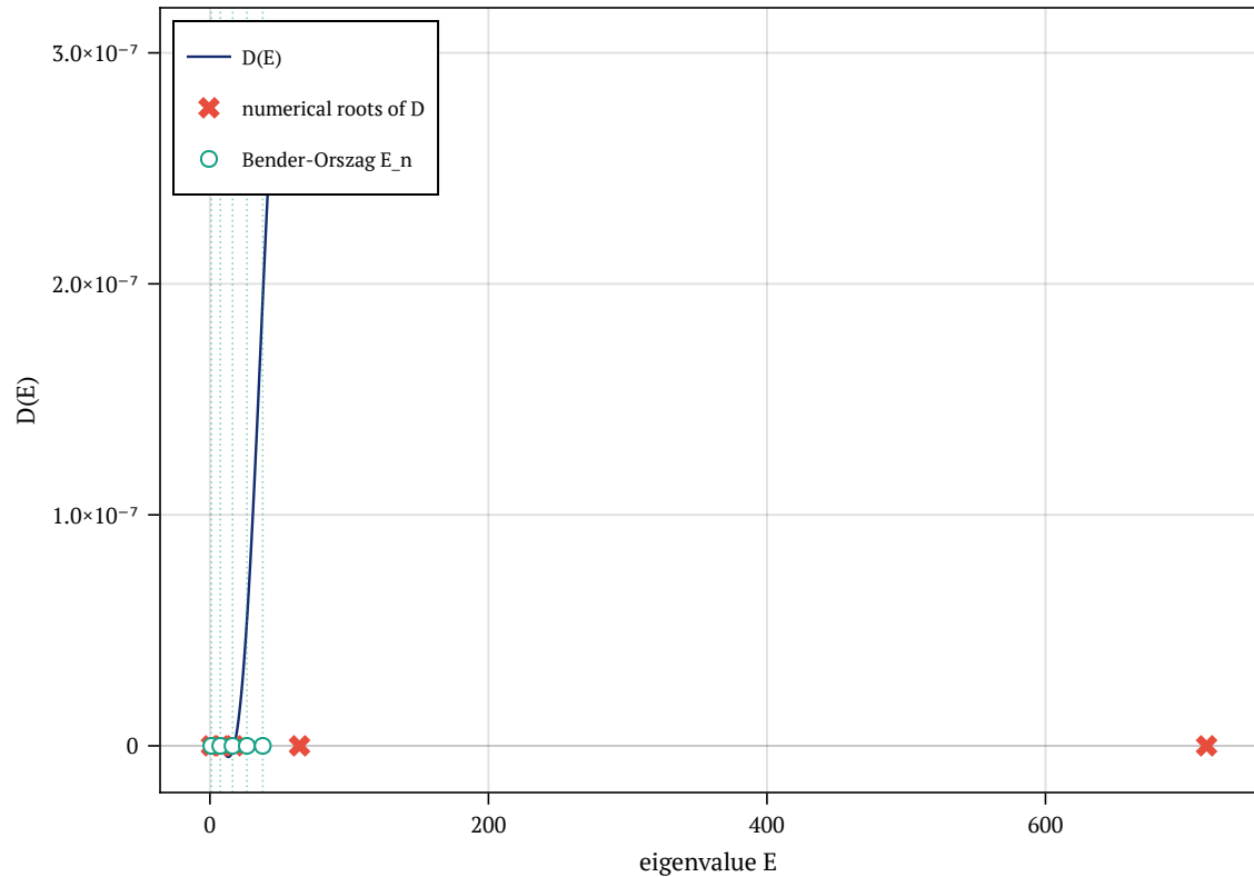
secular determinant D(E) and its roots
