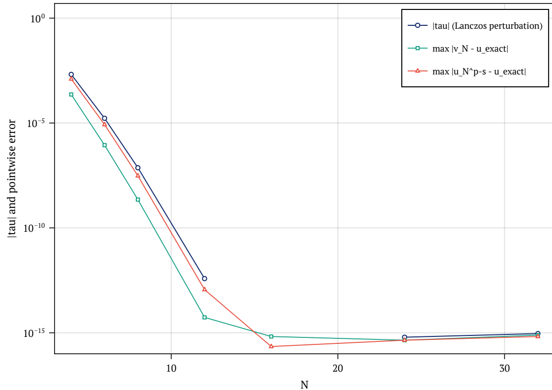
geometric decay of tau, geometric convergence
