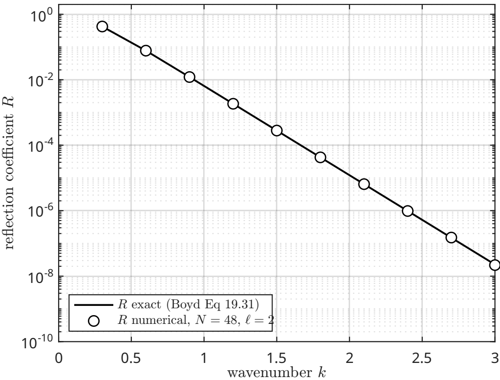
\text{sech}^2 scattering: spectral R matches the closed form
