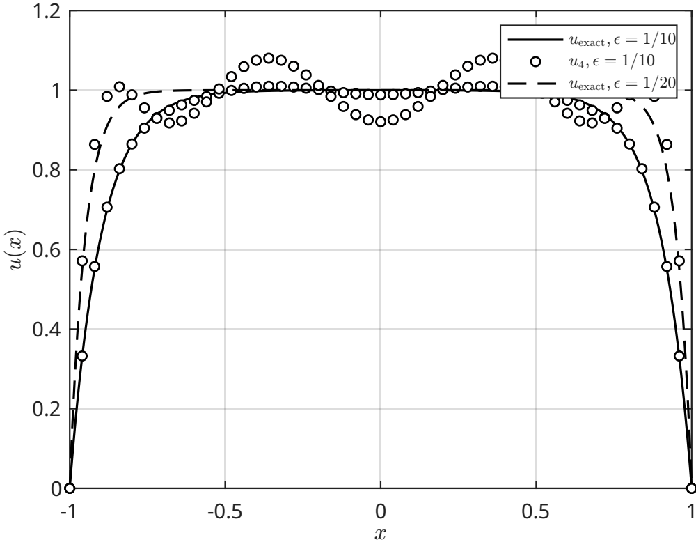
\epsilon^2 u'' - u = -1 : 4-term Galerkin vs exact
