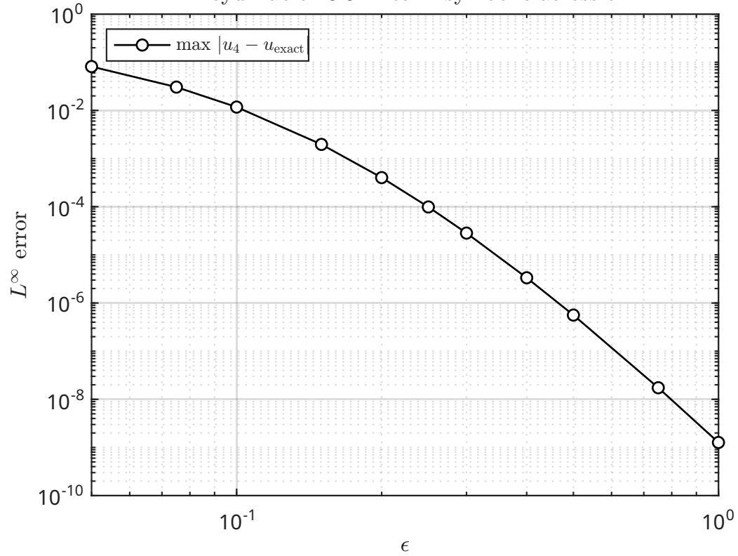
Boyd Table 20.3: 4-term symbolic across \epsilon
