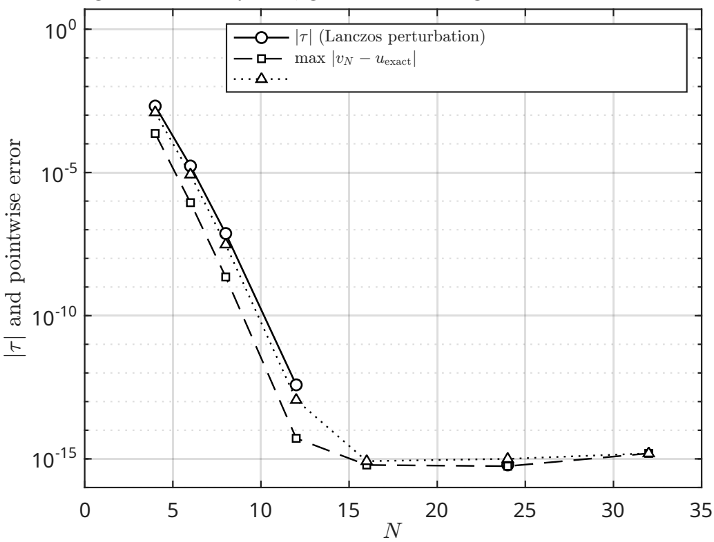
geometric decay of \tau , geometric convergence of both methods
