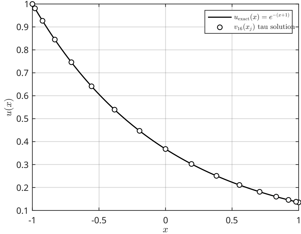
N = 16 : \tau \approx 0.000e + 00 , max err \approx 6.1e-16
