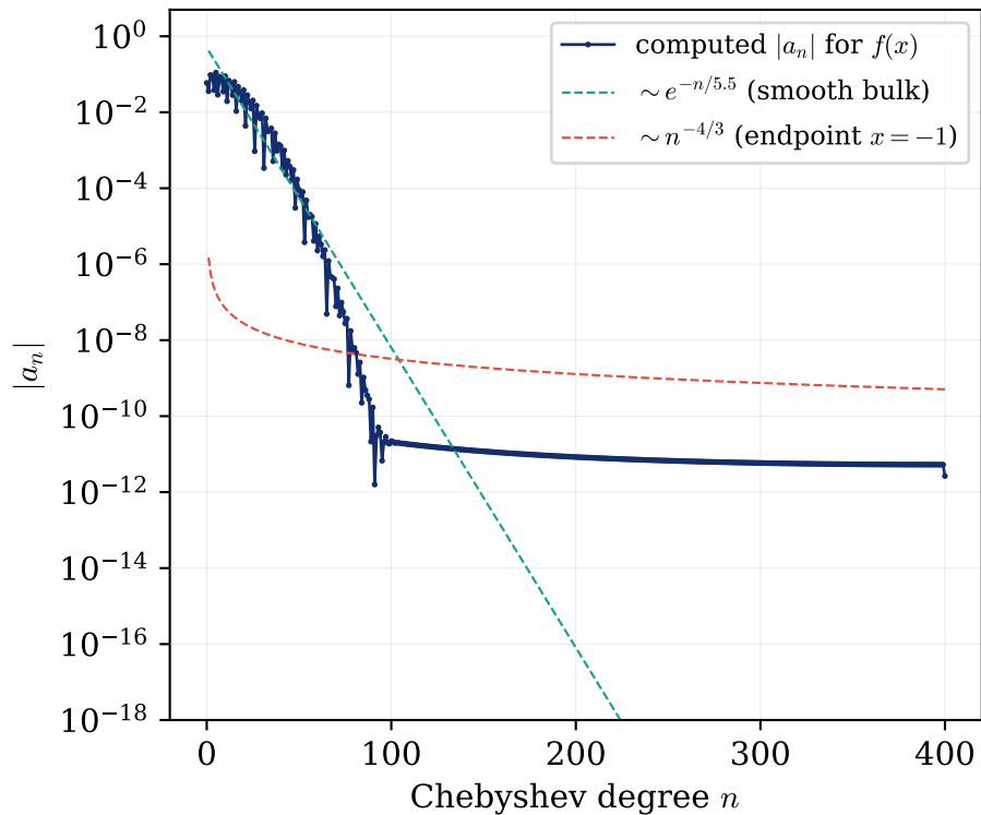
Panel B. f(x) = e^{-((x-0.3)/0.1)^2} + 10^{-7}(x+1)^{1/3}
