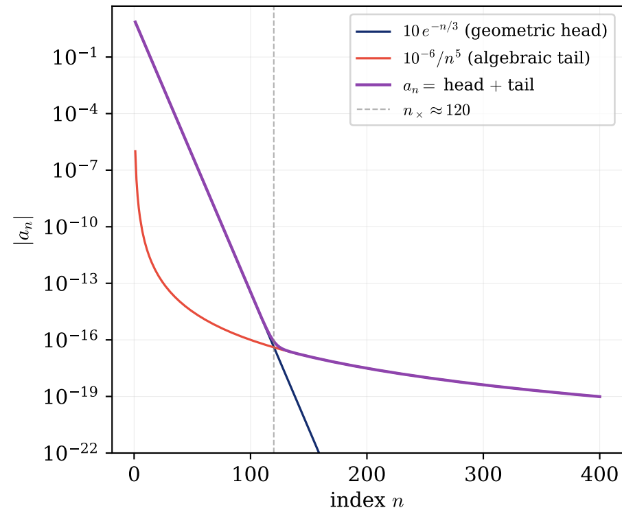
Panel A. Boyd's cartoon: a slope change at n_{\times}
