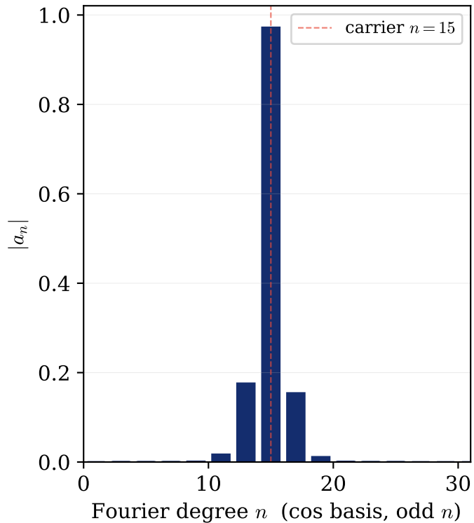
Panel A. |a_n| for ce_{15} at q = 10
