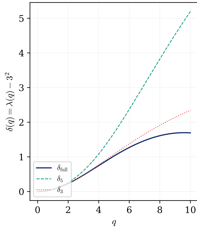
Panel C. ce_3 : q/n^2 large, sideband breaks
