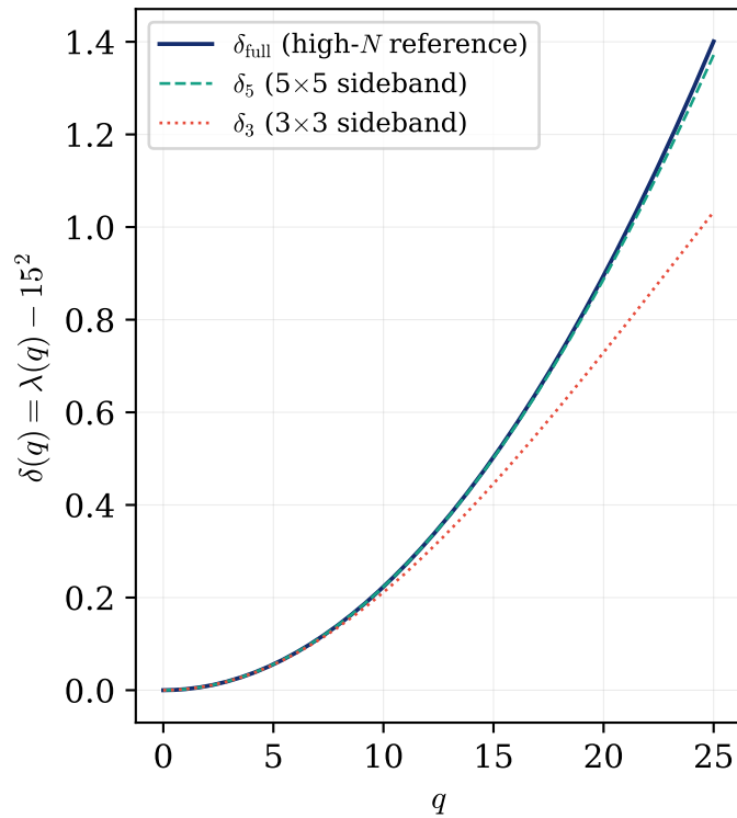
Panel B. ce_{15} : 5 \times 5 already exact at this scale
