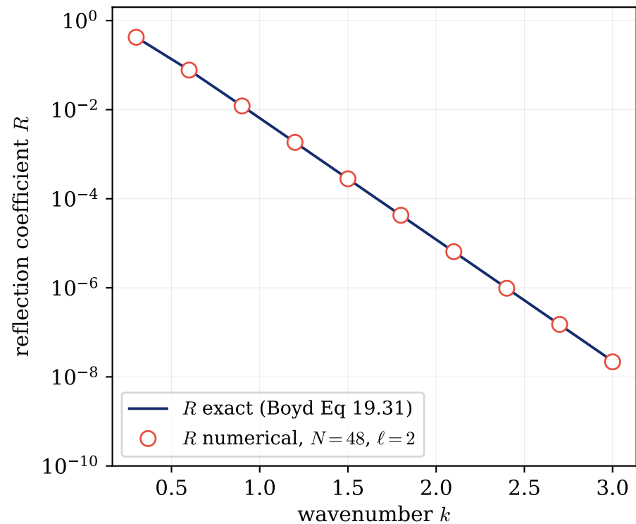
\text{sech}^2 scattering: spectral R matches the closed form
