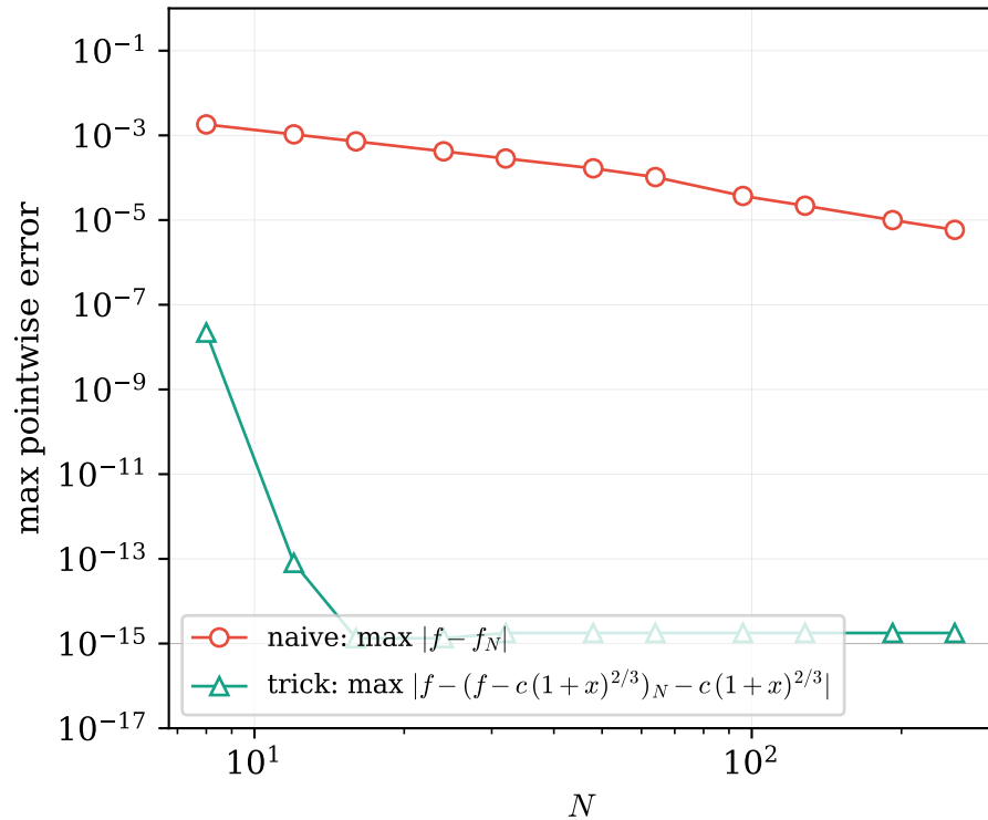
subtraction reaches machine \epsilon at modest N
