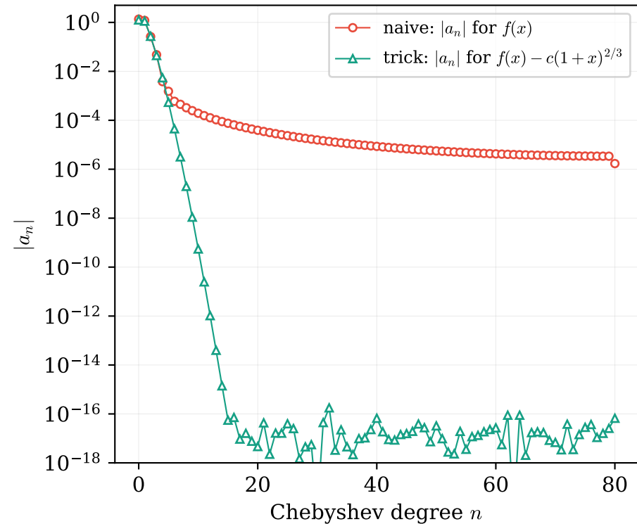
coefficient decay at N=80
