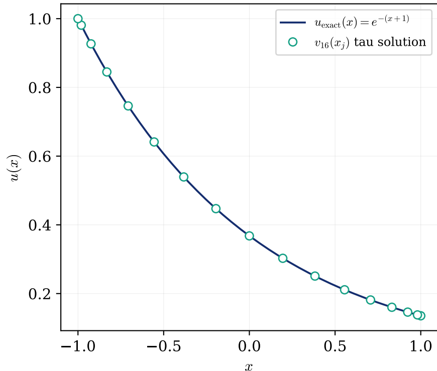
N = 16 : \tau \approx -4.722e-16 , max err \approx 5.6e-16
