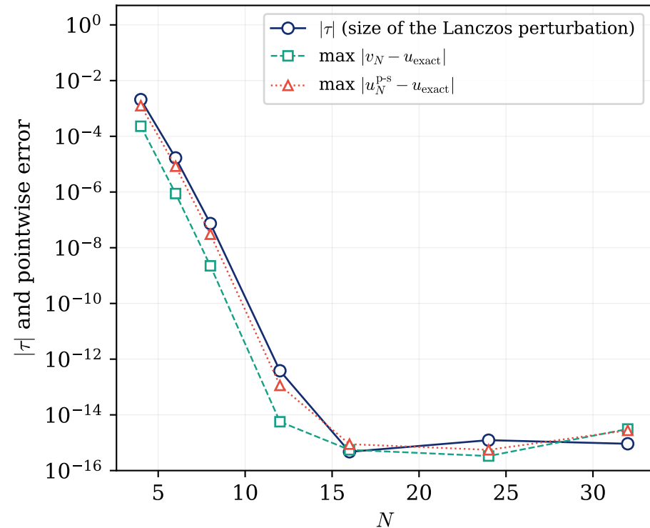
geometric decay of \tau , geometric convergence of both methods
