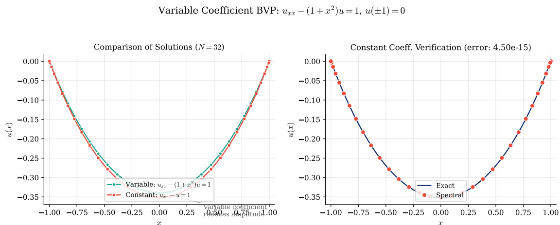
Figure 40: Variable coefficient BVP Equation 68. Left: comparison of solutions for variable coefficient (1 + x^2) and constant coefficient (1). The variable coefficient reduces the solution amplitude, especially near the boundaries where 1 + x^2 is largest. Right: verification of the constant-coefficient case against its exact solution.
