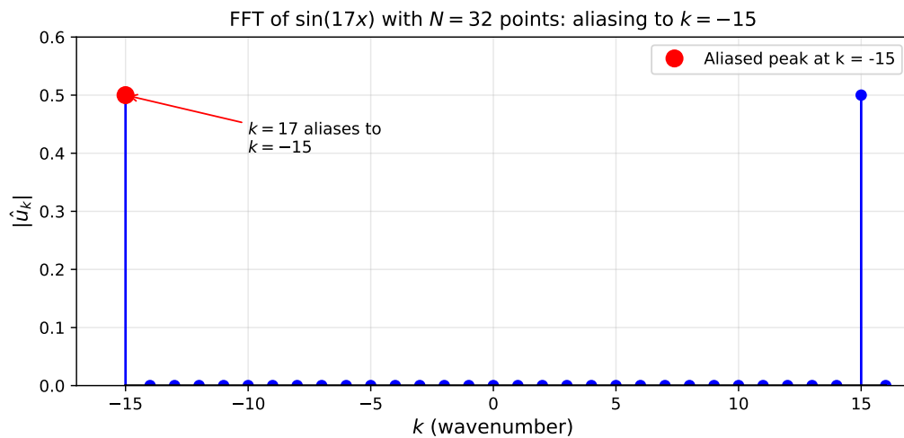
Figure 52: Aliasing in the FFT of \sin(17x) with N = 32 points. The true frequency k = 17 lies above the Nyquist limit N/2 = 16 . The FFT shows a spike at k = -15 because 17 = -15 + 32 : the frequency “wraps around” the Nyquist boundary.
