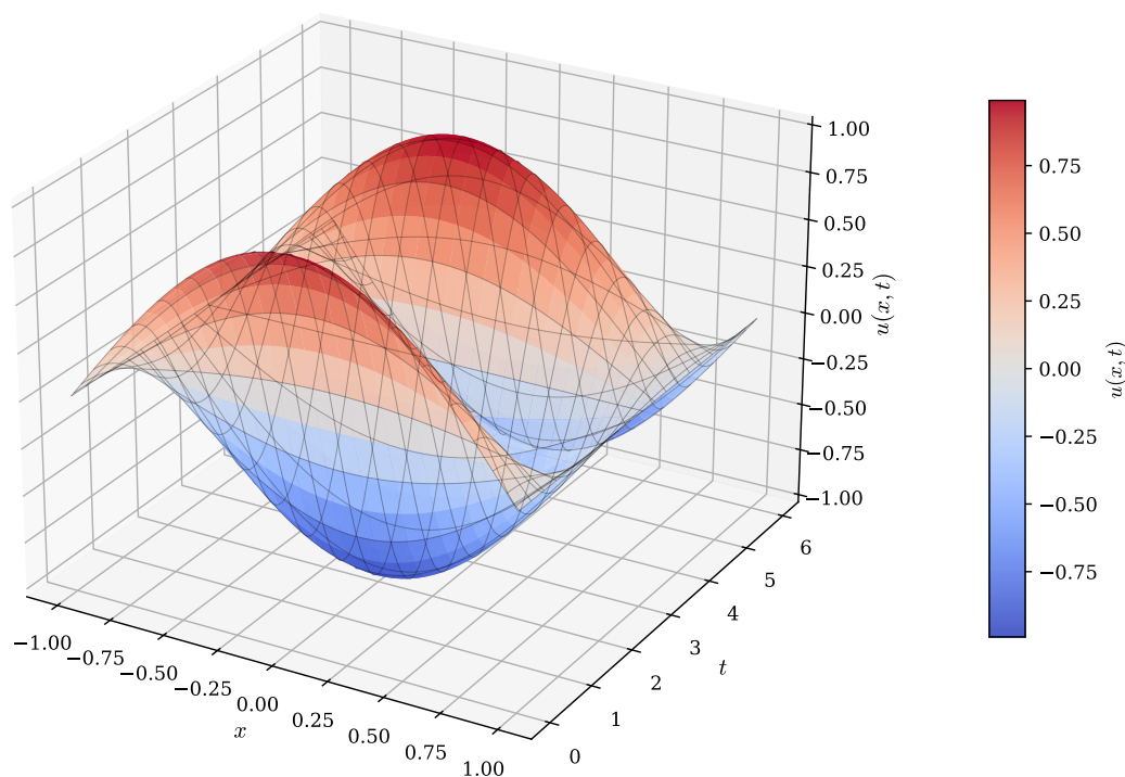
Figure 57: Solution of the 1D wave equation Equation 117 with initial half-sine profile. The waterfall plot shows u(x, t) for t \in [0, 6] . The initial shape splits into two counter-propagating waves, which reflect at the fixed boundaries ( x = \pm 1 ) with a sign change. The waves pass through each other and interfere, creating the characteristic standing wave pattern.
