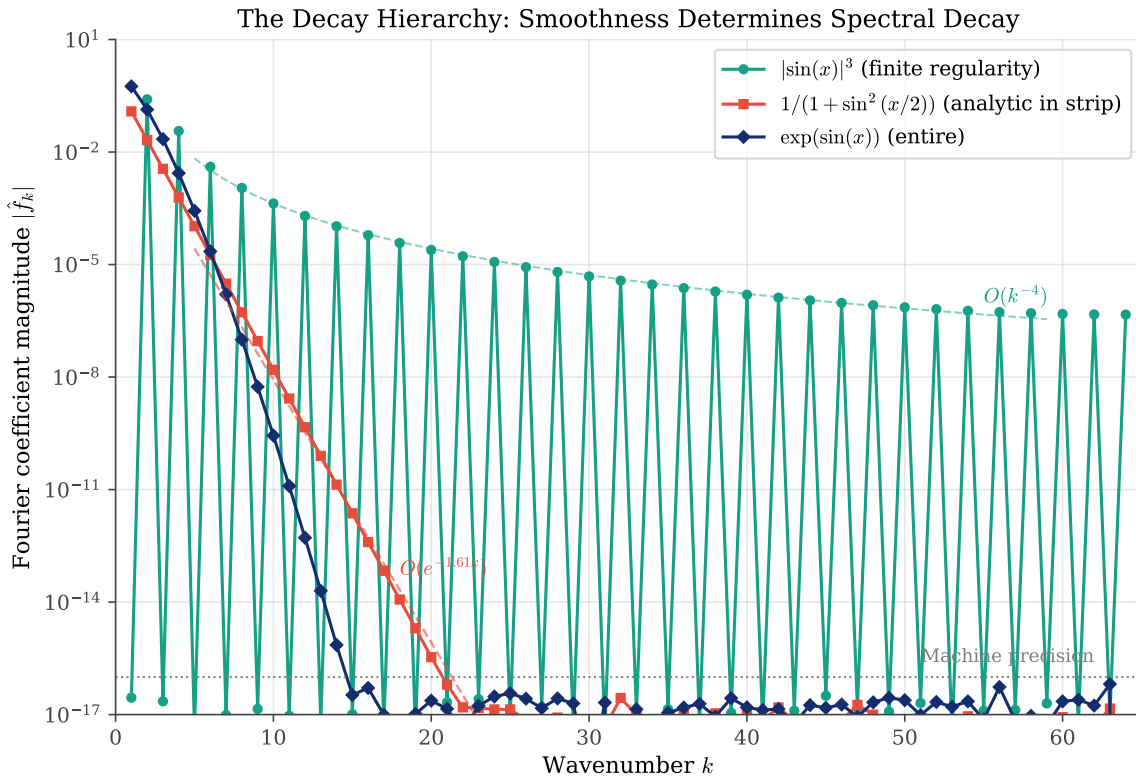
Figure 30: The decay hierarchy of Fourier coefficients. Functions with greater smoothness exhibit faster decay: algebraic ( O(k^{-4}) ) for finite regularity, geometric ( O(e^{-\alpha k}) ) for strip-analytic functions, and super-geometric for entire functions. The plot shows |\hat{f}_k| versus wavenumber k on a semi-log scale.
