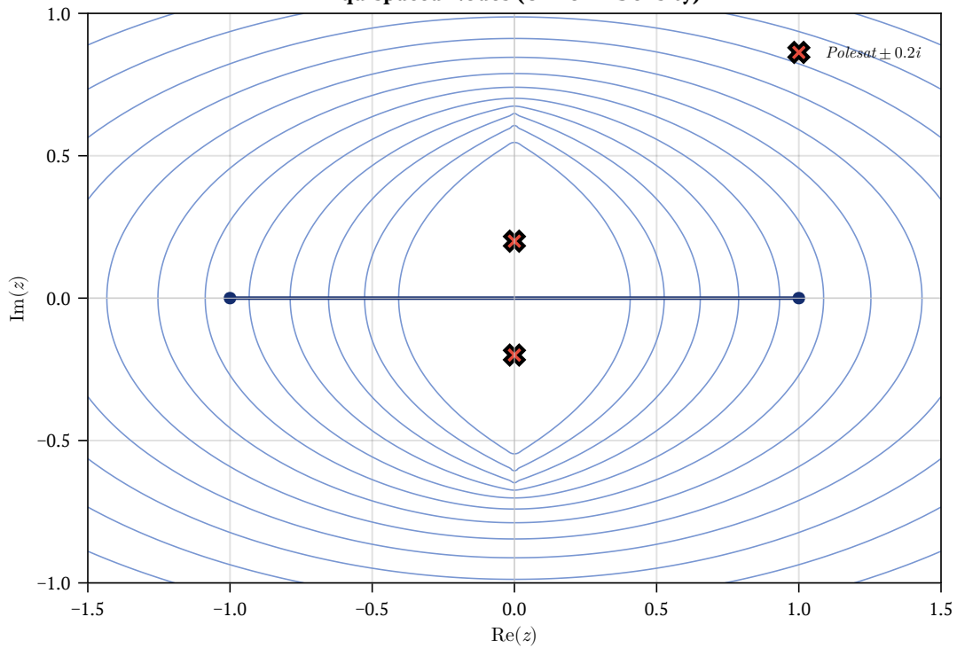
Equispaced Nodes (Uniform Density)
