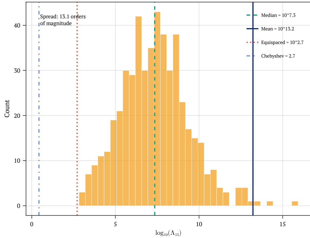
Distribution of \Lambda_N for N = 15 (500 trials)
