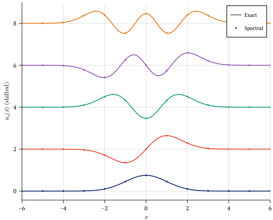
Harmonic Oscillator Eigenfunctions (N=64, L=8)
