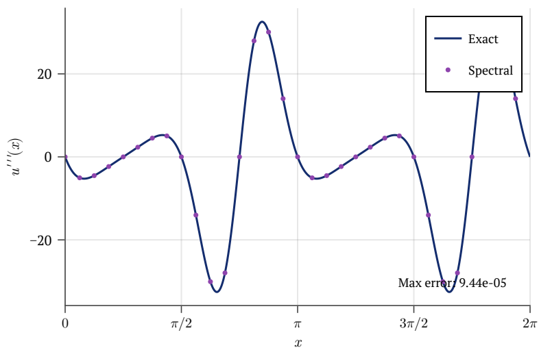
Third derivative
