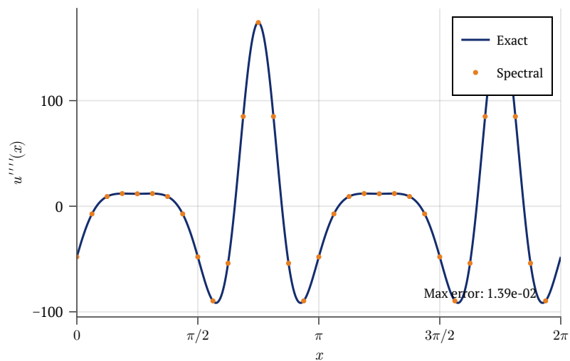
Fourth derivative
