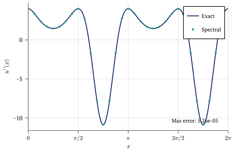
Second derivative
