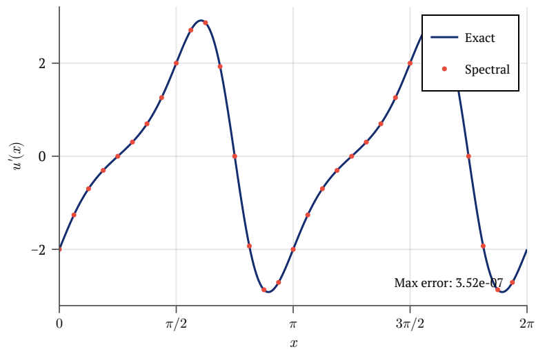
First derivative
