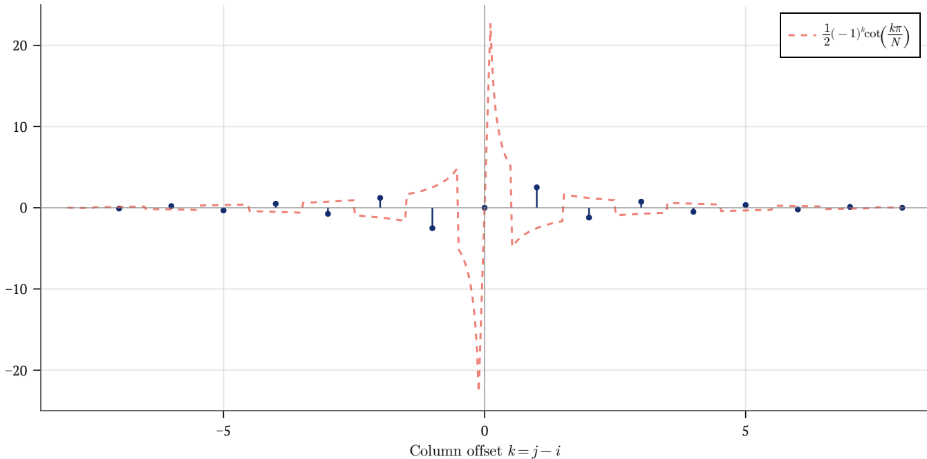
First Row Profile (Toeplitz Structure)
