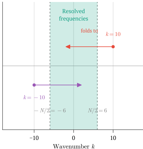
Frequency Folding ( N=12 )
