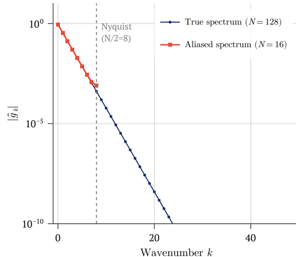
True vs. Aliased Spectrum
