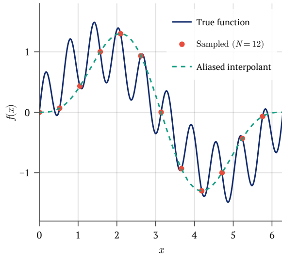
Coarse Sampling Misses High Frequencies
