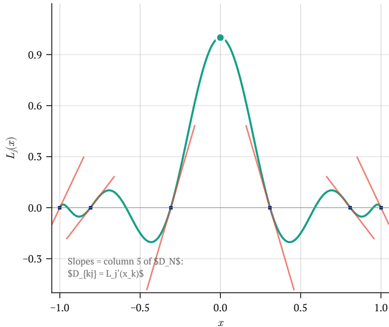
Cardinal Function L_5 with Derivative Slopes
