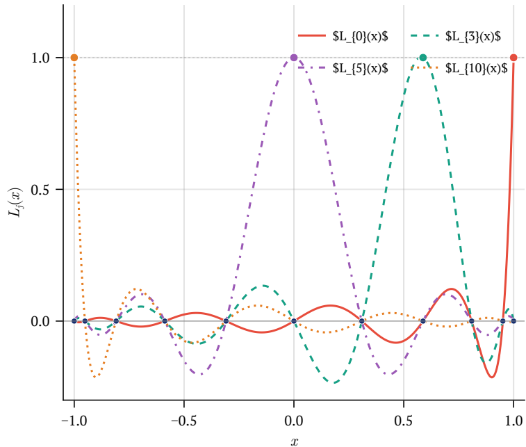
Chebyshev Cardinal Functions ($N = 10$)
