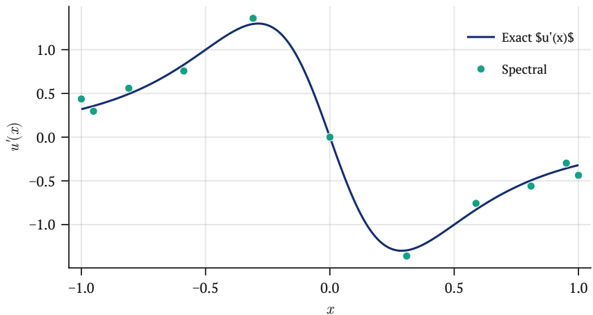
Derivative with N = 10 (max error: 1.16e-01)
