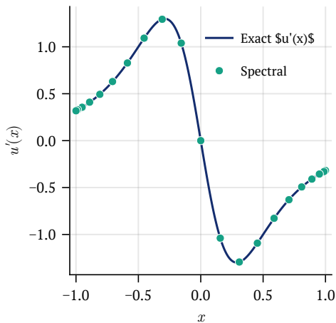
Derivative with N = 20 (max error: 1.89e-02)
