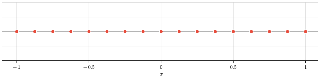
Equispaced Grid ($N = 16$ intervals)
