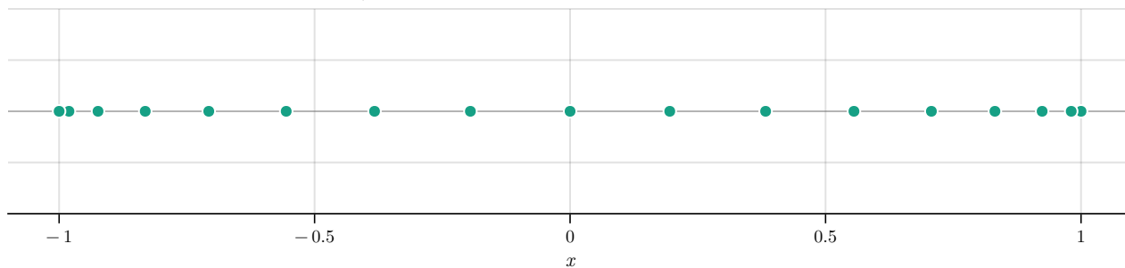
Chebyshev-Gauss-Lobatto Grid ($N = 16$ intervals)
