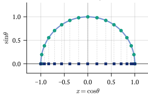
Circle Projection: x_j = \cos(j\pi/N)
