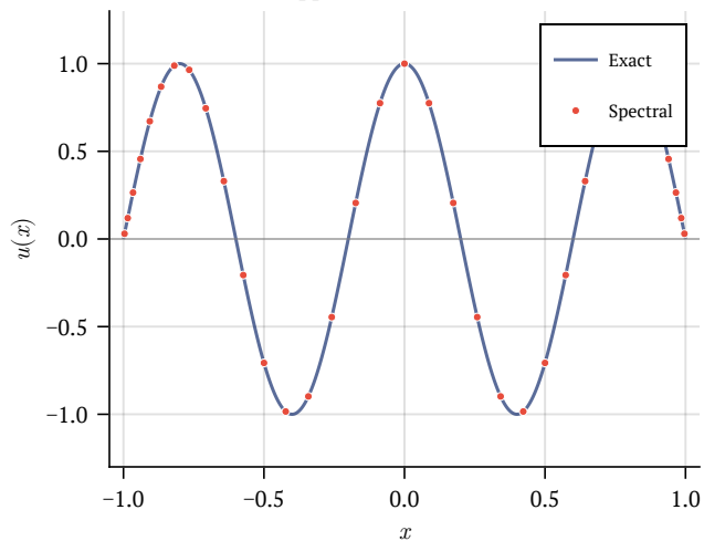
Mode 5: ppw = 14.4, \lambda error = 9.2\text{e-}16
