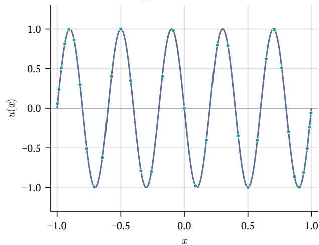
Mode 10: ppw = 7.2, \lambda error = 2.3\text{e-}13
