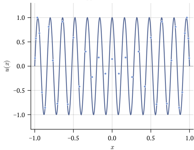
Mode 25: ppw = 2.9, \lambda error = 1.6\text{e-}02
