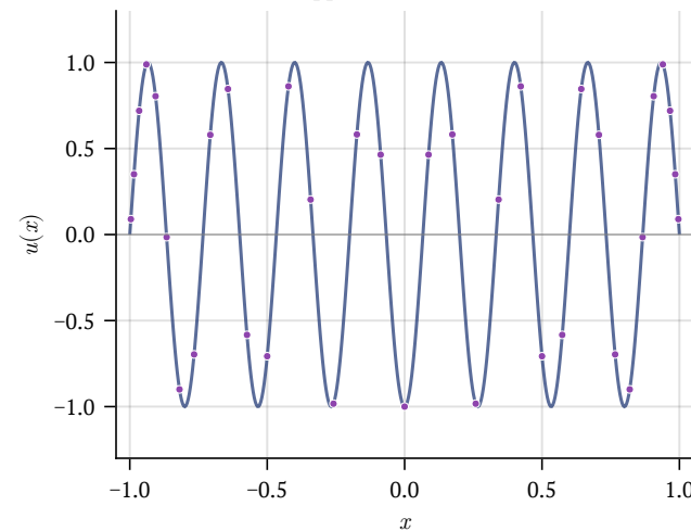
Mode 15: ppw = 4.8, \lambda error = 3.6\text{e-}08
