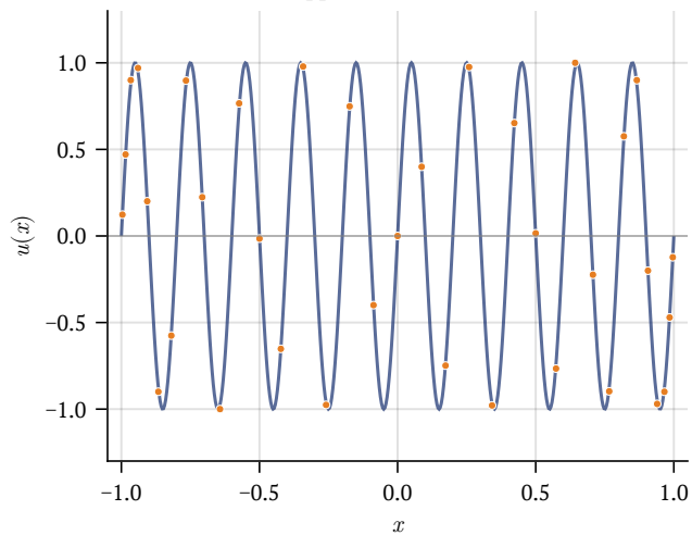
Mode 20: ppw = 3.6, \lambda error = 1.1\text{e-}03
