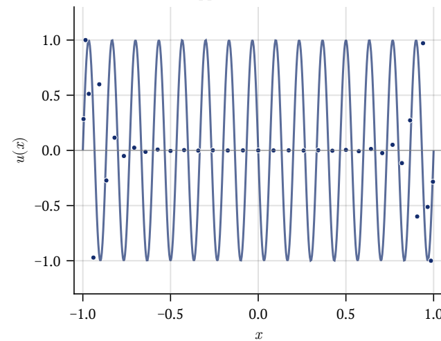
Mode 30: ppw = 2.4, \lambda error = 1.6\text{e+}00
