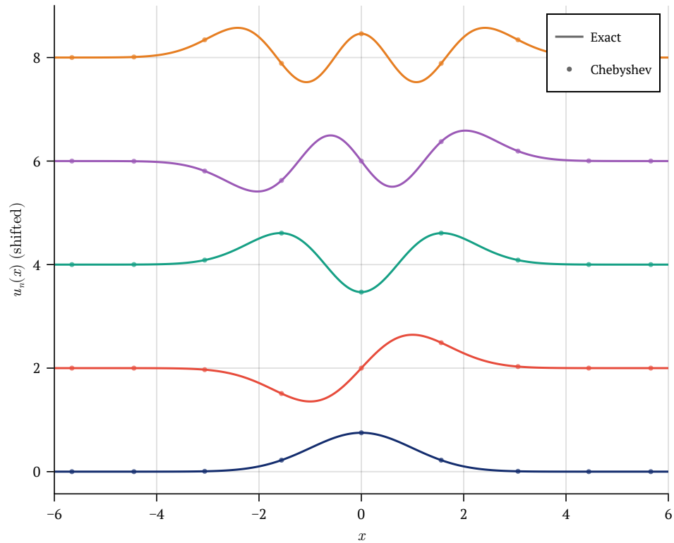
Chebyshev Eigenfunctions (N=64, L=8)
