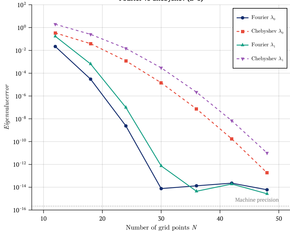
Fourier vs Chebyshev (L=8)
