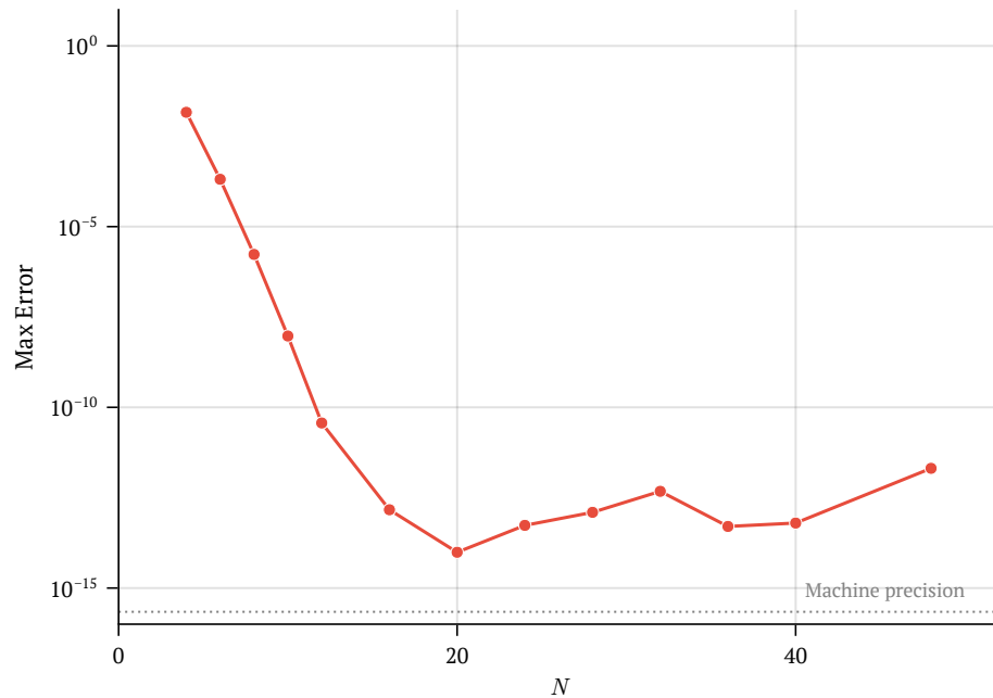
Convergence
