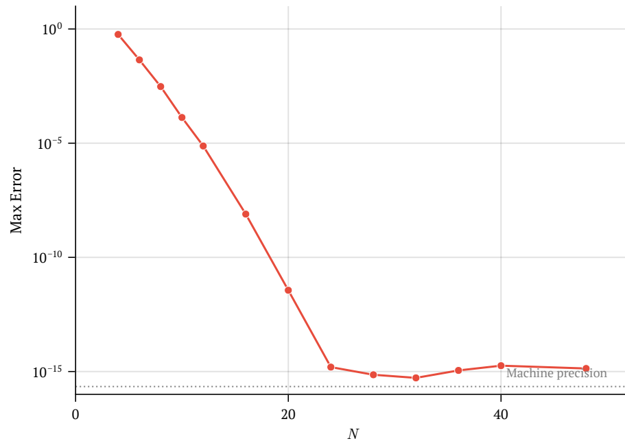
Convergence
