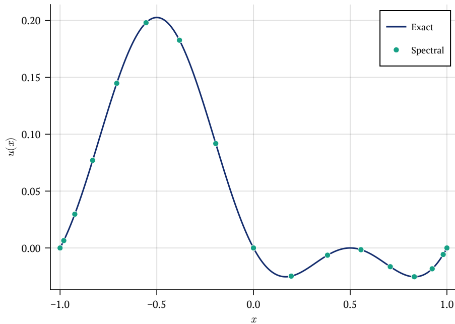
Solution (N = 16, max error: 7.84e-09)
