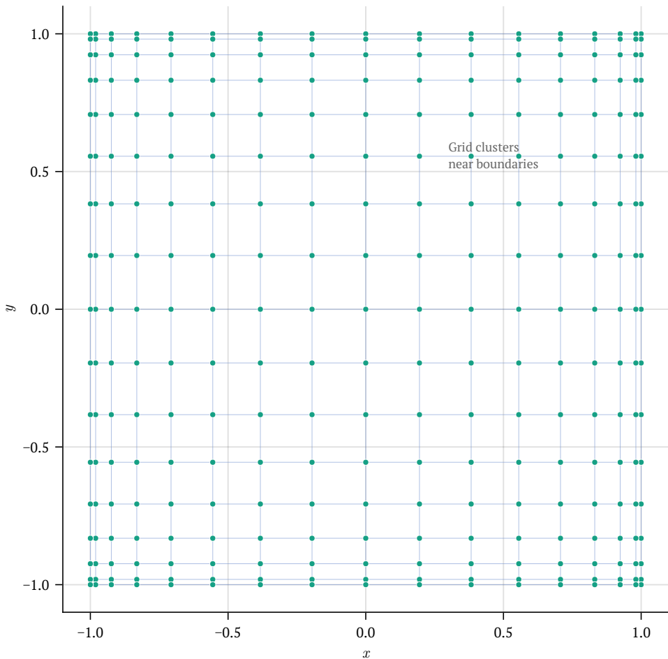
Chebyshev Tensor Product Grid (N = 16)
