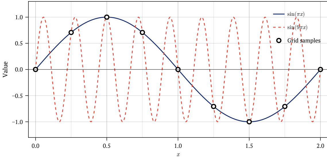
Aliasing on grid h = 1/4 : \sin(\pi x) and \sin(9\pi x) coincide
