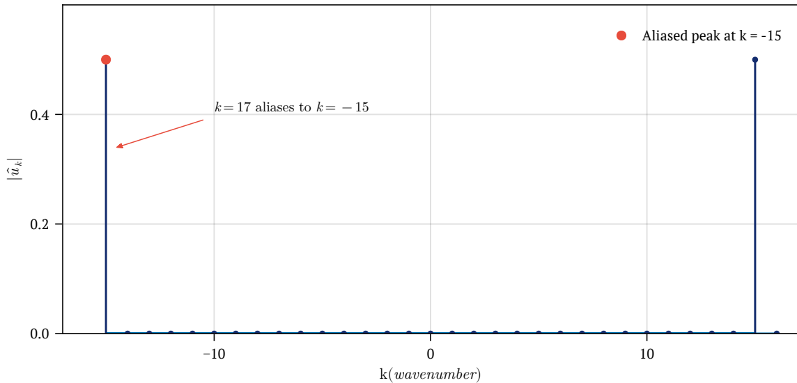
FFT of \sin(17x) with N=32 points: aliasing to k=-15
