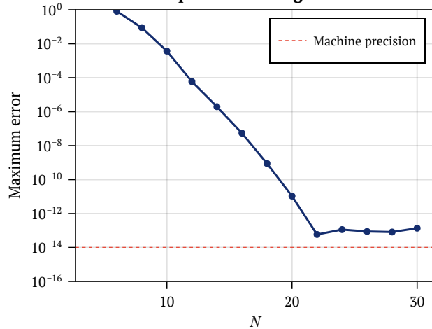
Spectral convergence
