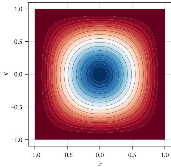
Exact Solution
