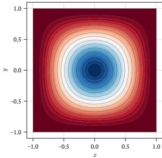
Numerical Solution
