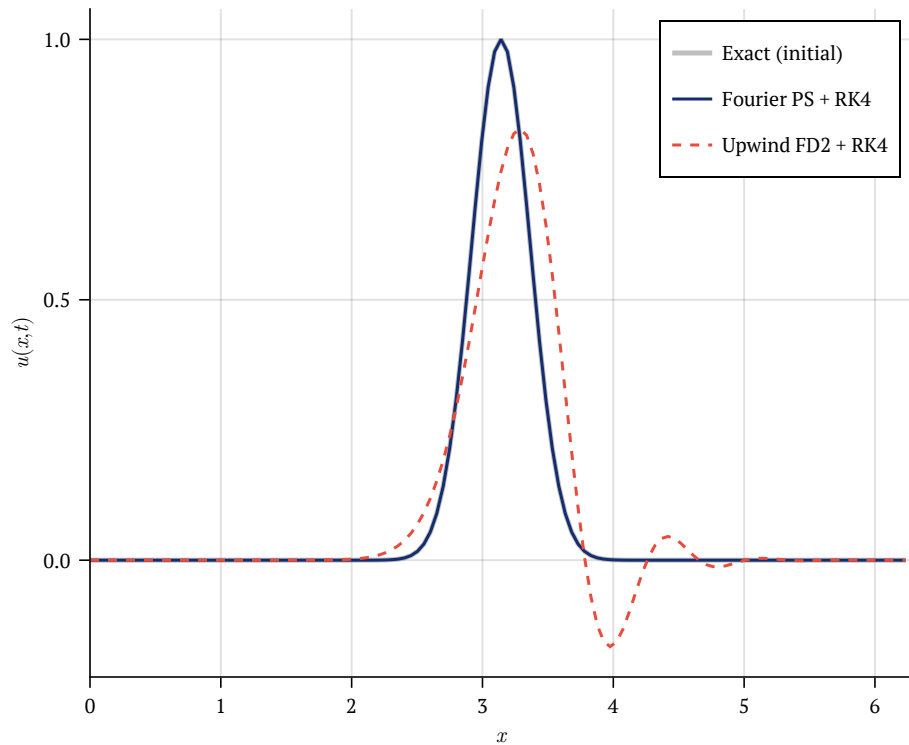
After one period ( t = 2\pi / c , N = 128 )
