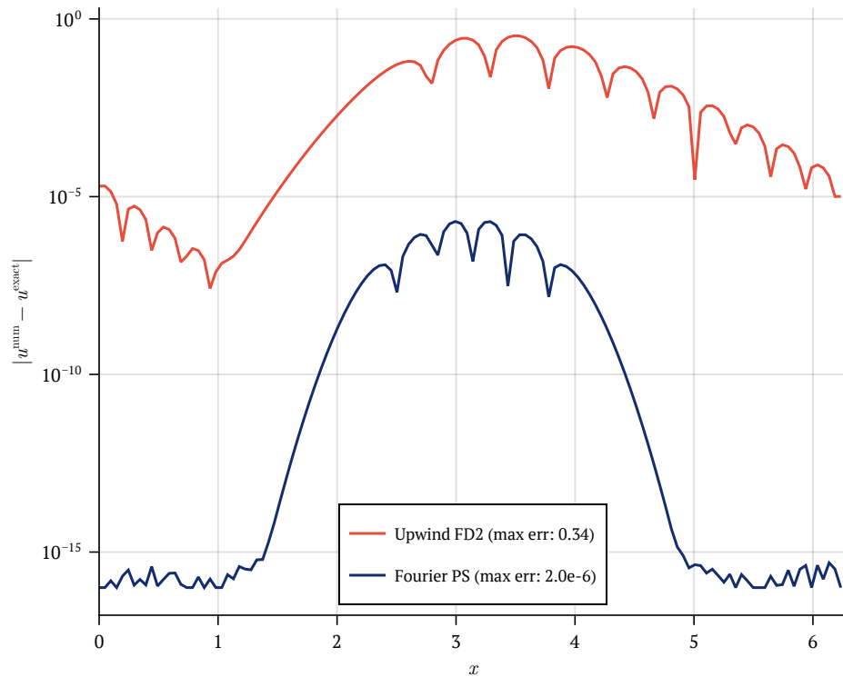
Pointwise Error After One Period
