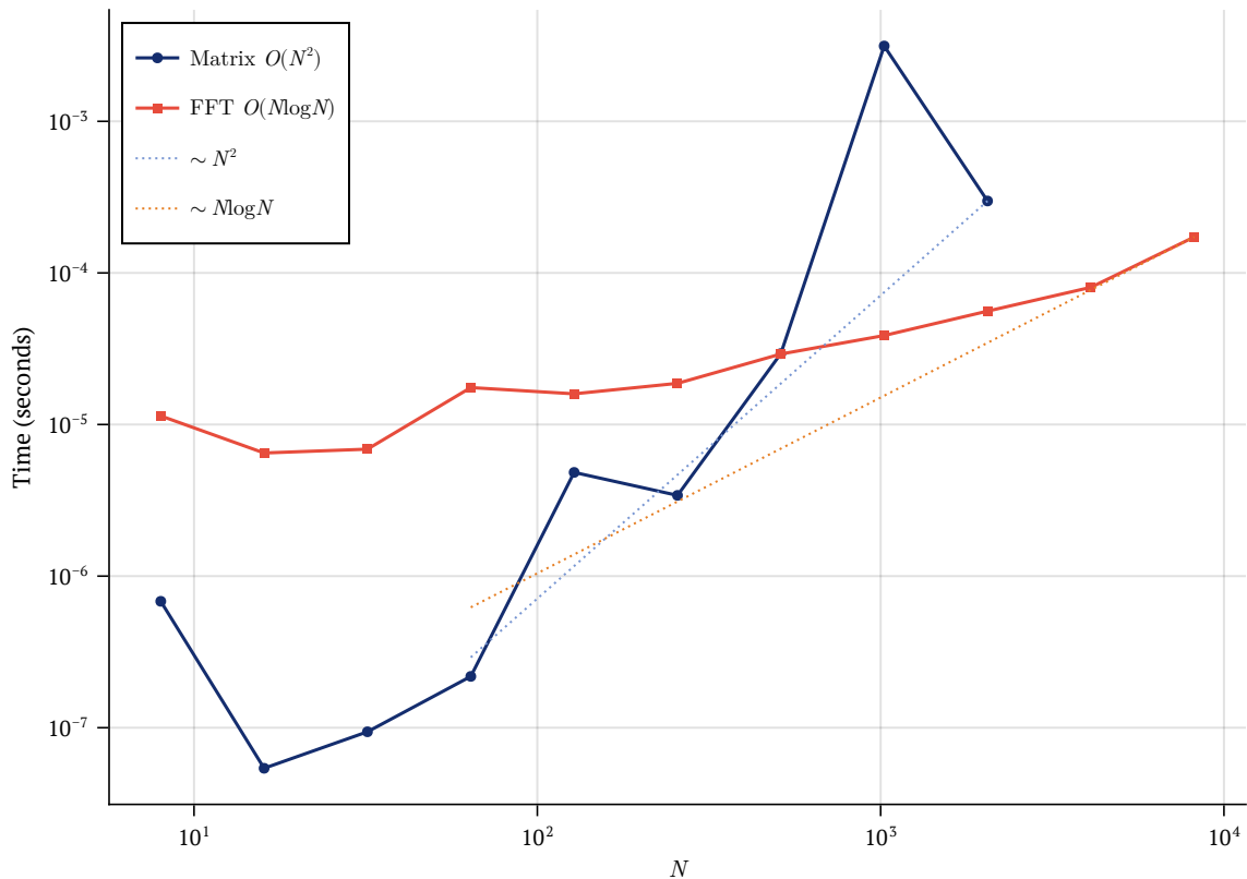
Computational Cost: Matrix vs FFT Differentiation
