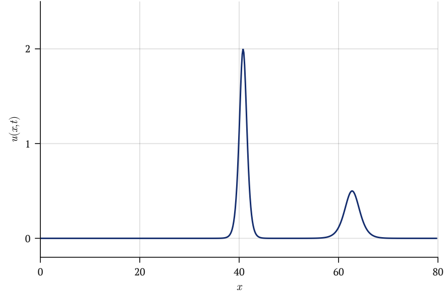
After collision ( t = 25 )
