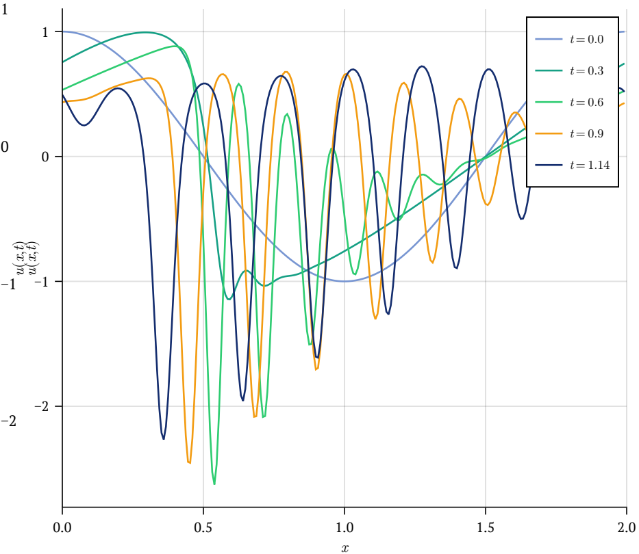
Soliton Train Formation
