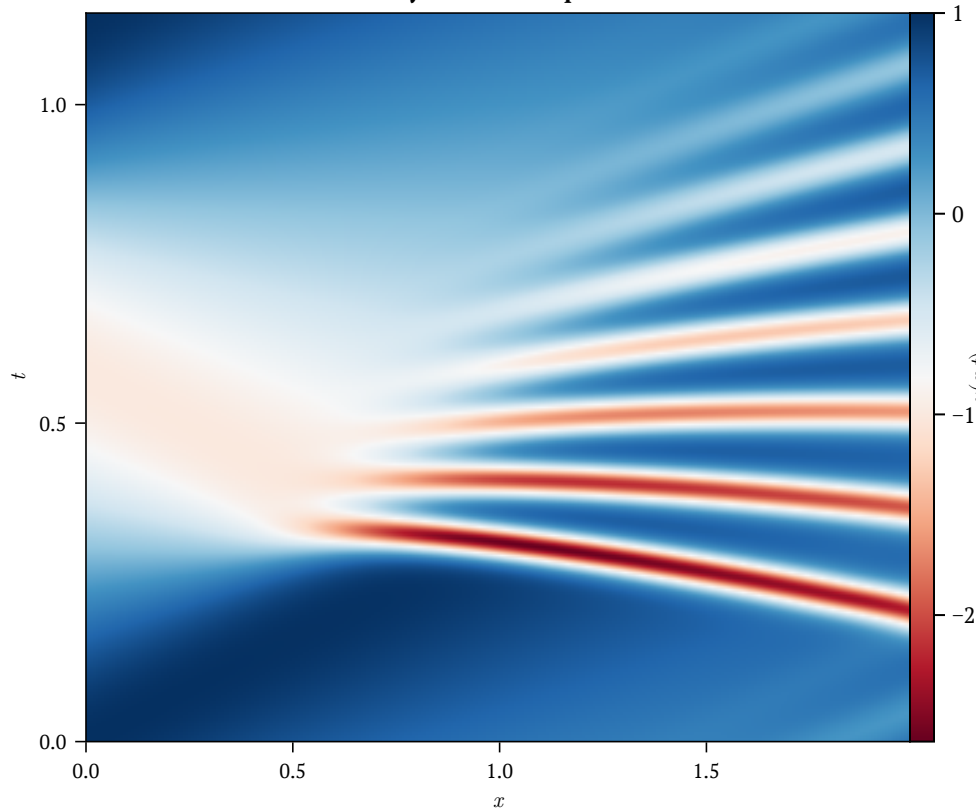
Zabusky--Kruskal Experiment
