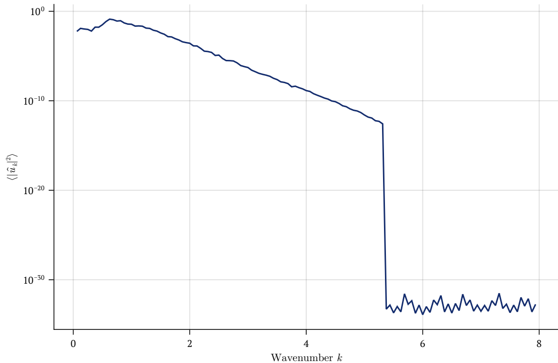
Time-Averaged Energy Spectrum (KS)
