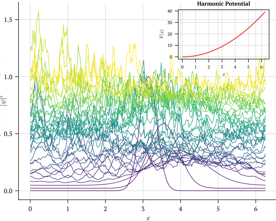
Waterfall View: |\psi|^2 Evolution
