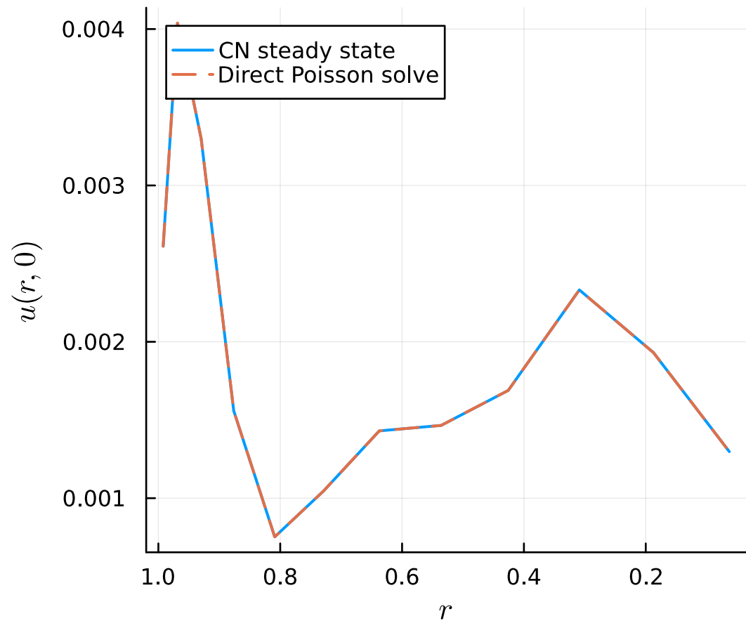
Steady state vs Poisson solution (theta = 0)
