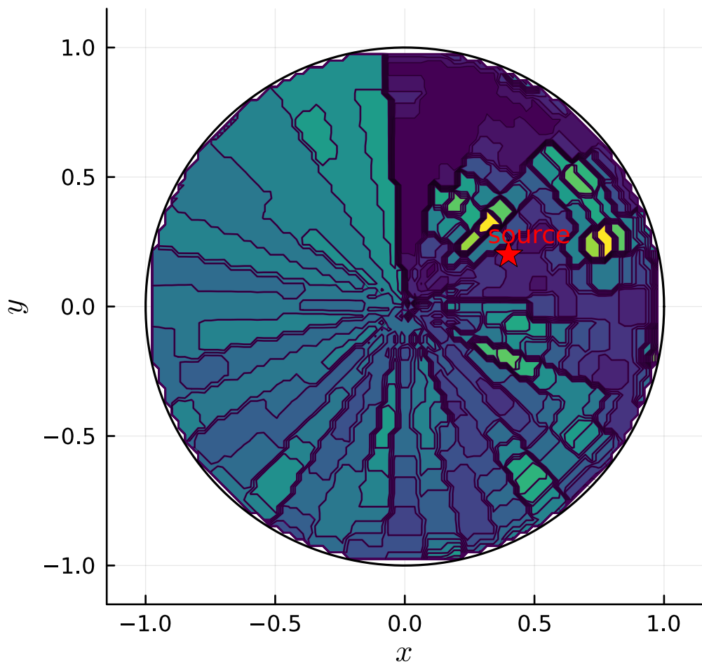
Poisson solution: filled contour
