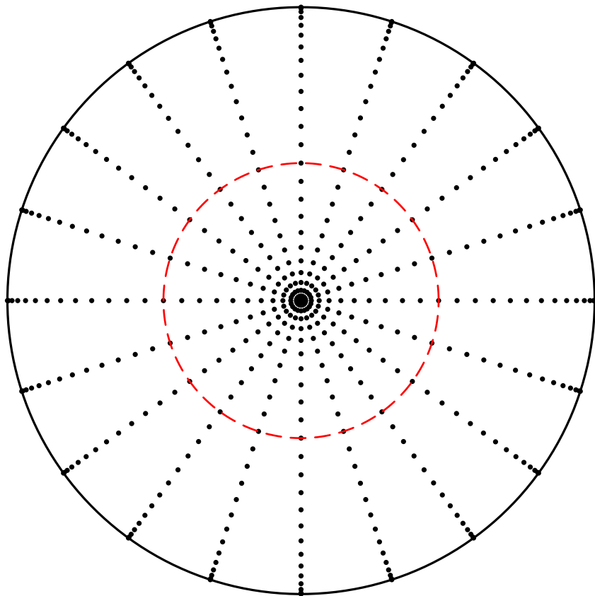
Naive grid ( r in [0, 1] ) Median circle: 22% of area
