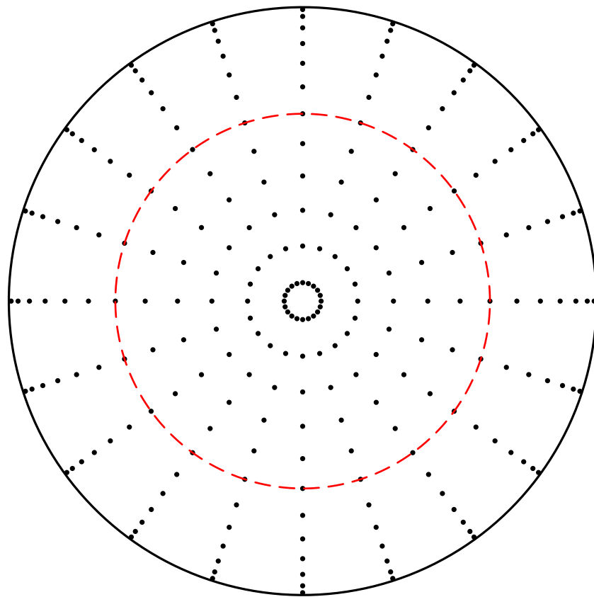
Doubled grid ( r in [-1, 1] ) Median circle: 41% of area
