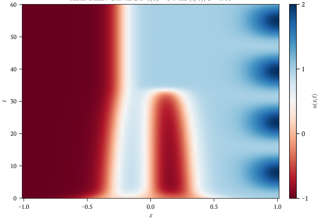
Allen-Cahn : Driven BC u(1) = 1 + \sin^2(t/5) , \varepsilon = 0.01
